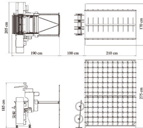
場地規劃 Installation layout
