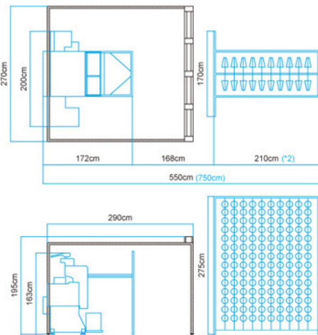
場地規劃 Installation layout
